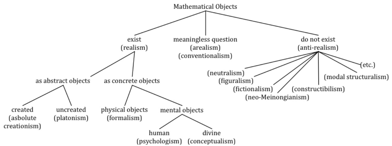
Fig. 1: Some options concerning the existence of mathematical objects.
